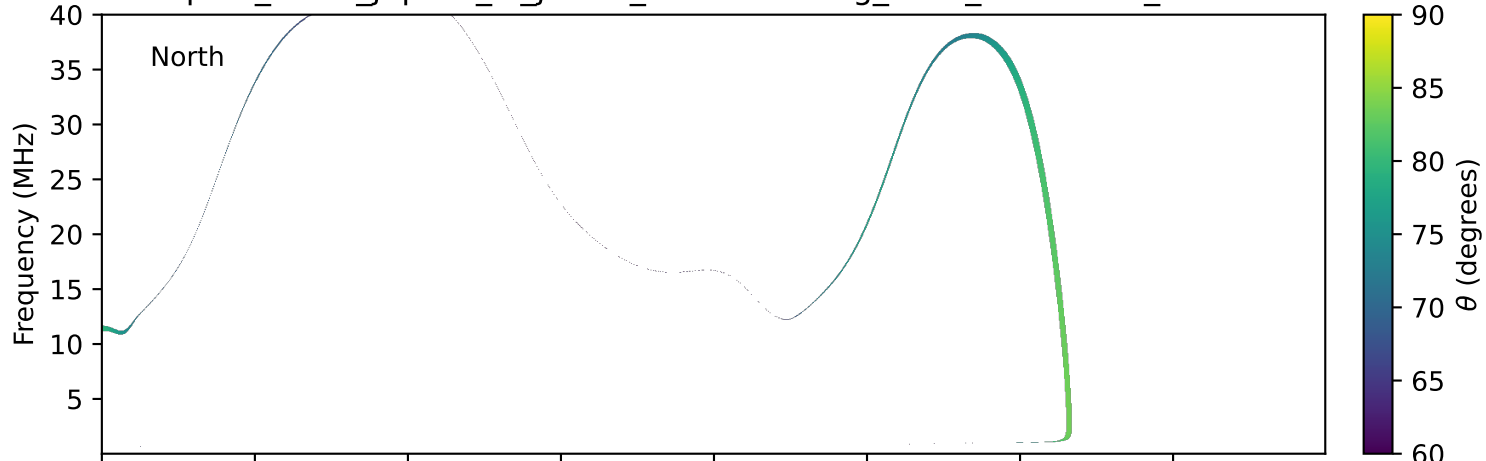
expres_earth_jupiter_io_jrm33_lossc-wid1deg_3kev_19981214_v11.cdf
