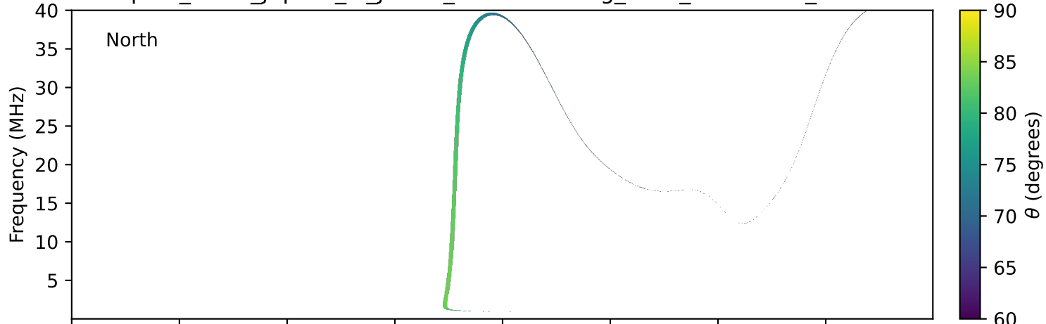
expres_earth_jupiter_io_jrm33_lossc-wid1deg_3kev_19981210_v11.cdf
