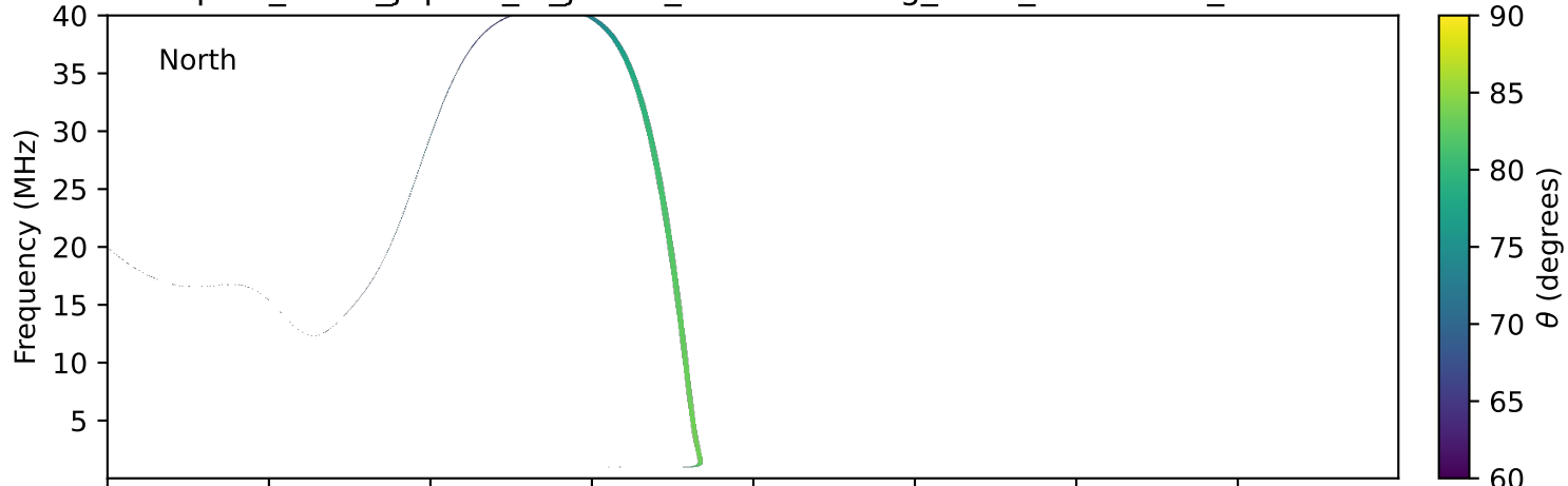
expres_earth_jupiter_io_jrm33_lossc-wid1deg_3kev_19981209_v11.cdf
