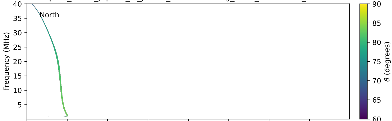
expres_earth_jupiter_io_jrm33_lossc-wid1deg_3kev_19981204_v11.cdf
