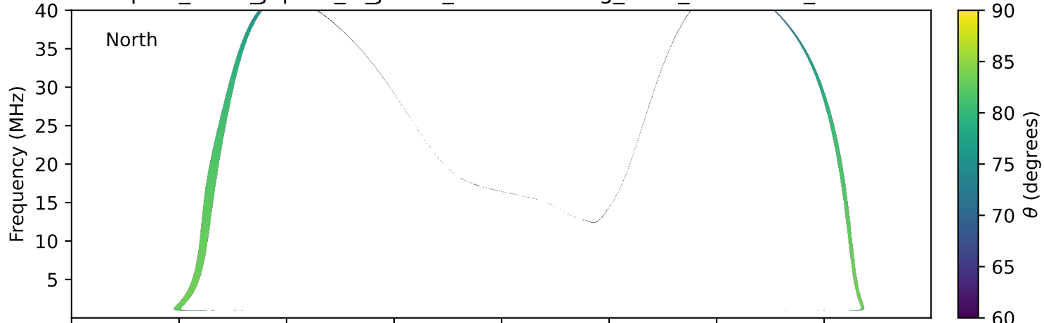
expres_earth_jupiter_io_jrm09_lossc-wid1deg_3kev_19981228_v11.cdf
