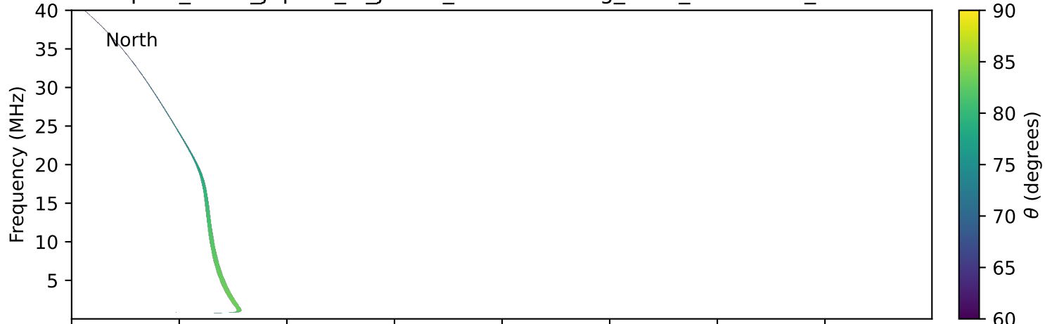
expres_earth_jupiter_io_jrm09_lossc-wid1deg_3kev_19981211_v11.cdf
