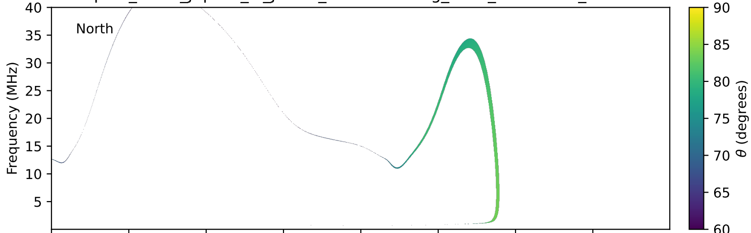
expres_earth_jupiter_io_jrm09_lossc-wid1deg_3kev_19981207_v11.cdf
