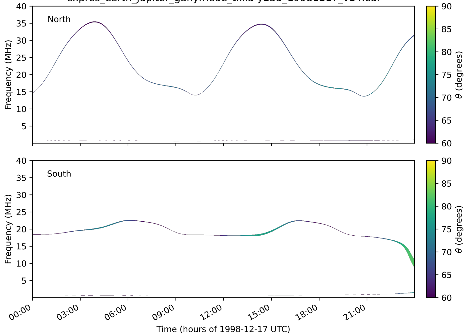
expres_earth_jupiter_ganymede_txka-y235_19981217_v14.cdf
