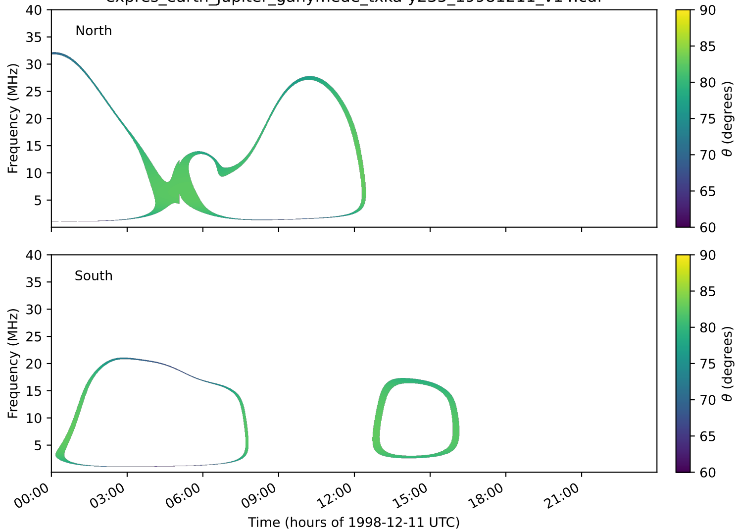
expres_earth_jupiter_ganymede_txka-y235_19981211_v14.cdf
