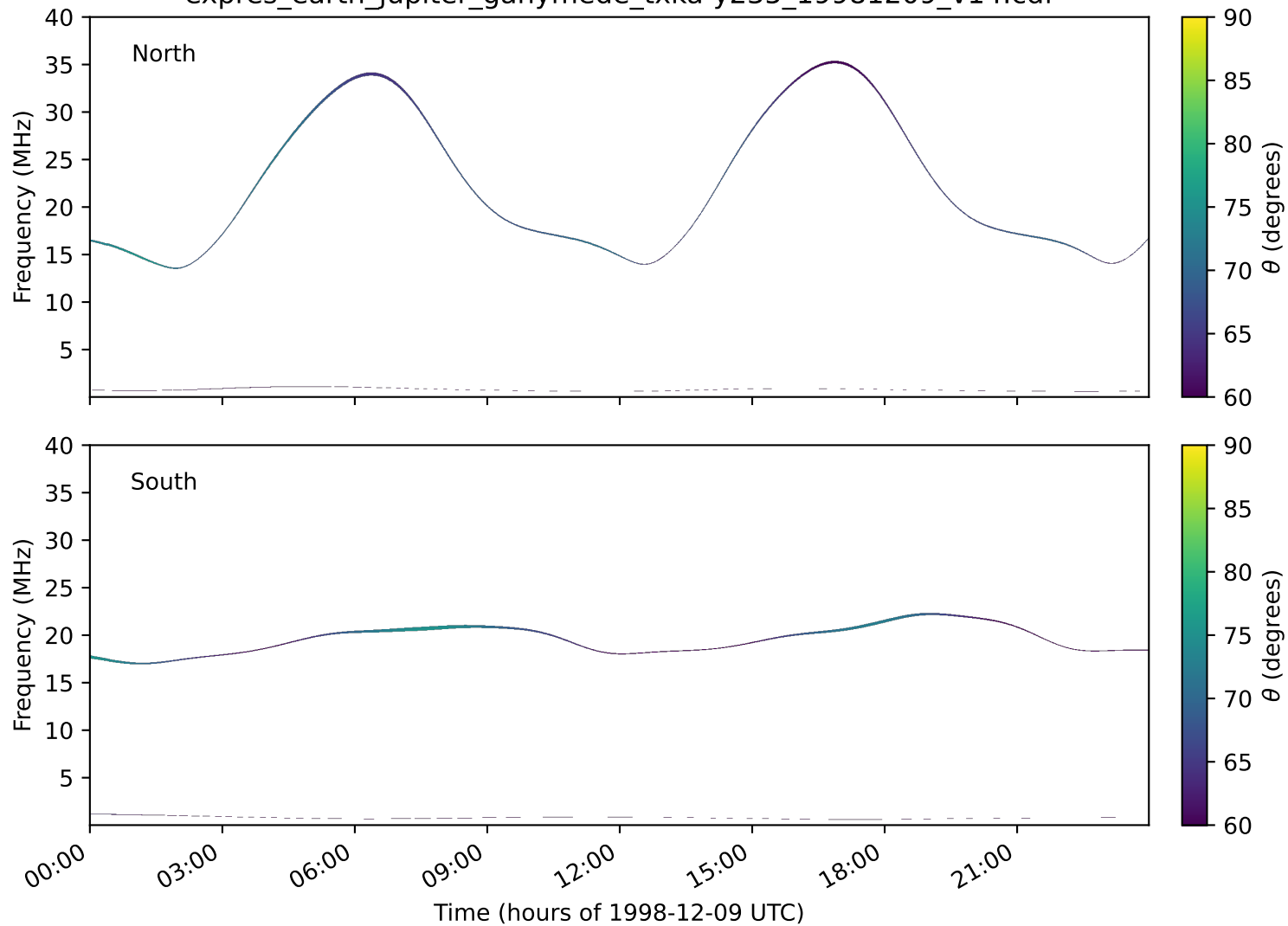
expres_earth_jupiter_ganymede_txka-y235_19981209_v14.cdf
