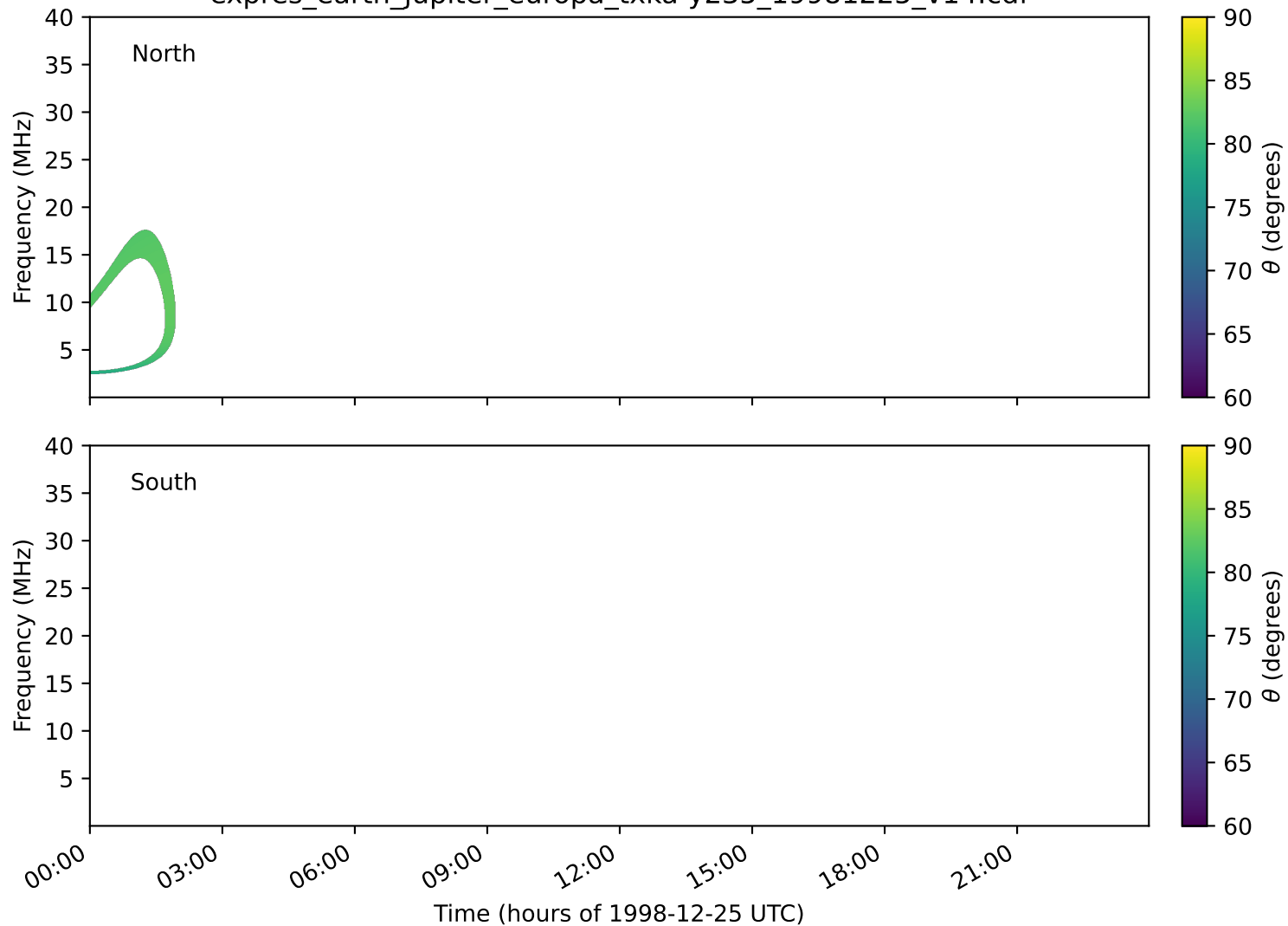
expres_earth_jupiter_europa_txka-y235_19981225_v14.cdf
