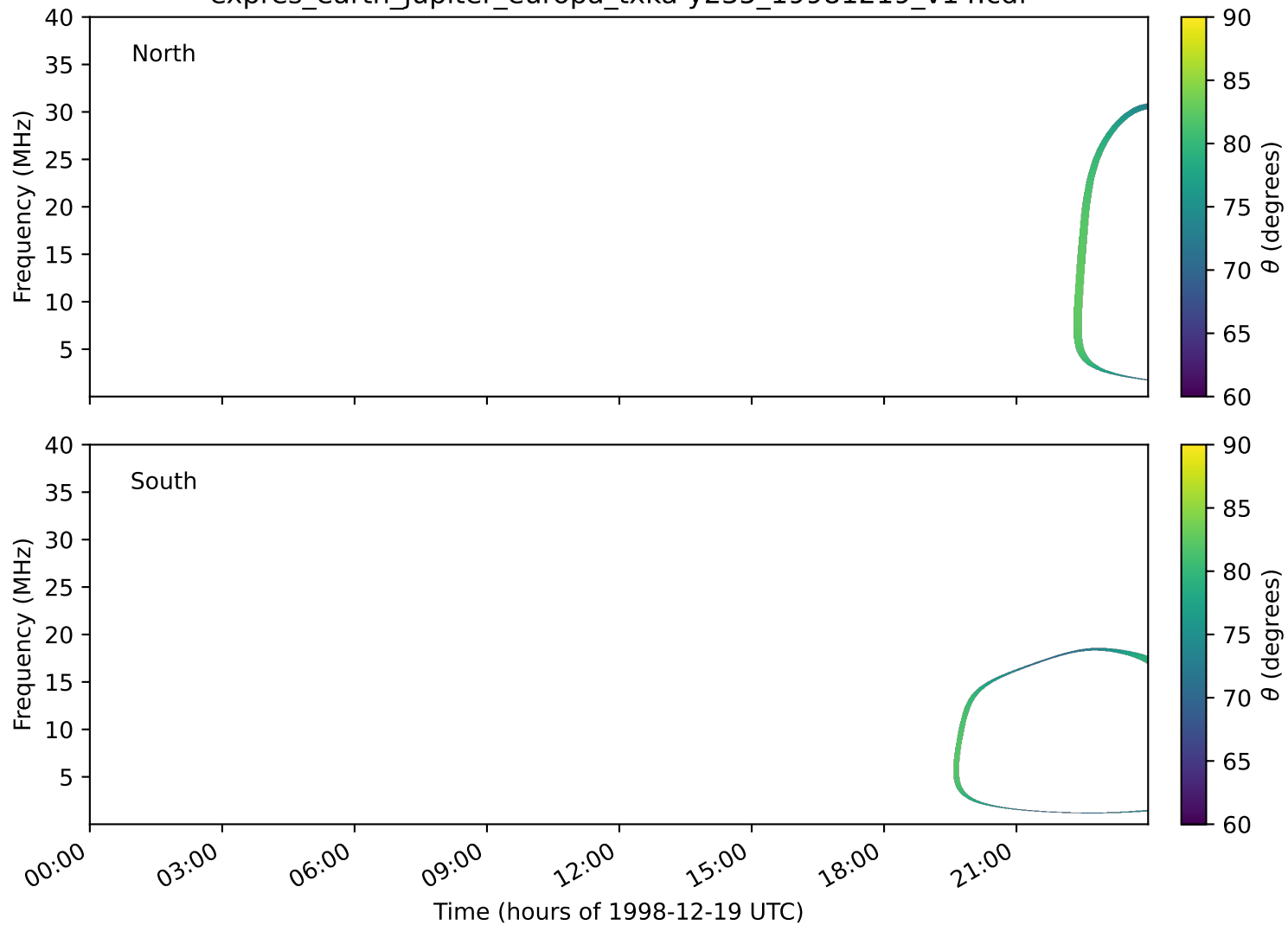
expres_earth_jupiter_europa_txka-y235_19981219_v14.cdf
