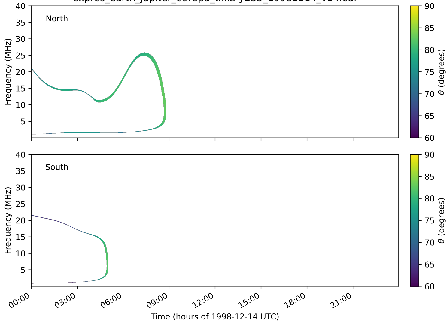
expres_earth_jupiter_europa_txka-y235_19981214_v14.cdf
