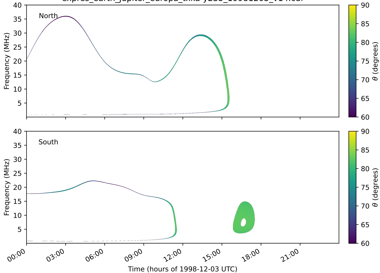
expres_earth_jupiter_europa_txka-y235_19981203_v14.cdf
