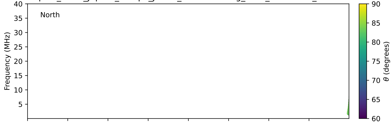
expres_earth_jupiter_europa_jrm33_lossc-wid1deg_3kev_19981226_v11.cdf
