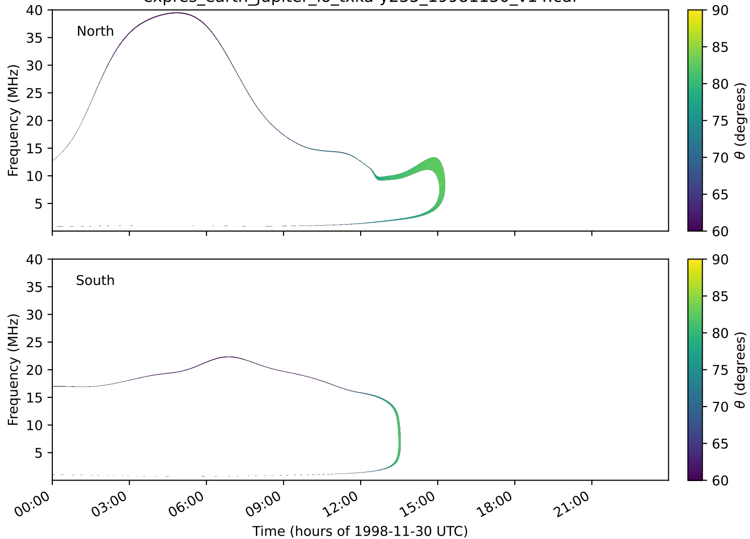
expres_earth_jupiter_io_txka-y235_19981130_v14.cdf
