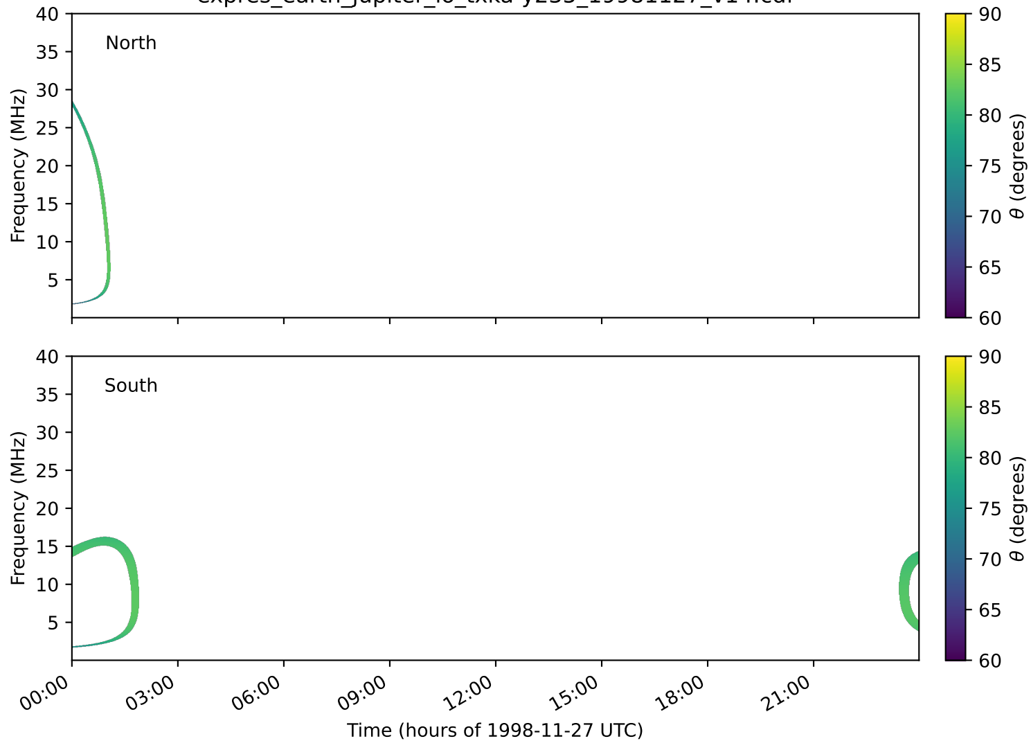
expres_earth_jupiter_io_txka-y235_19981127_v14.cdf
