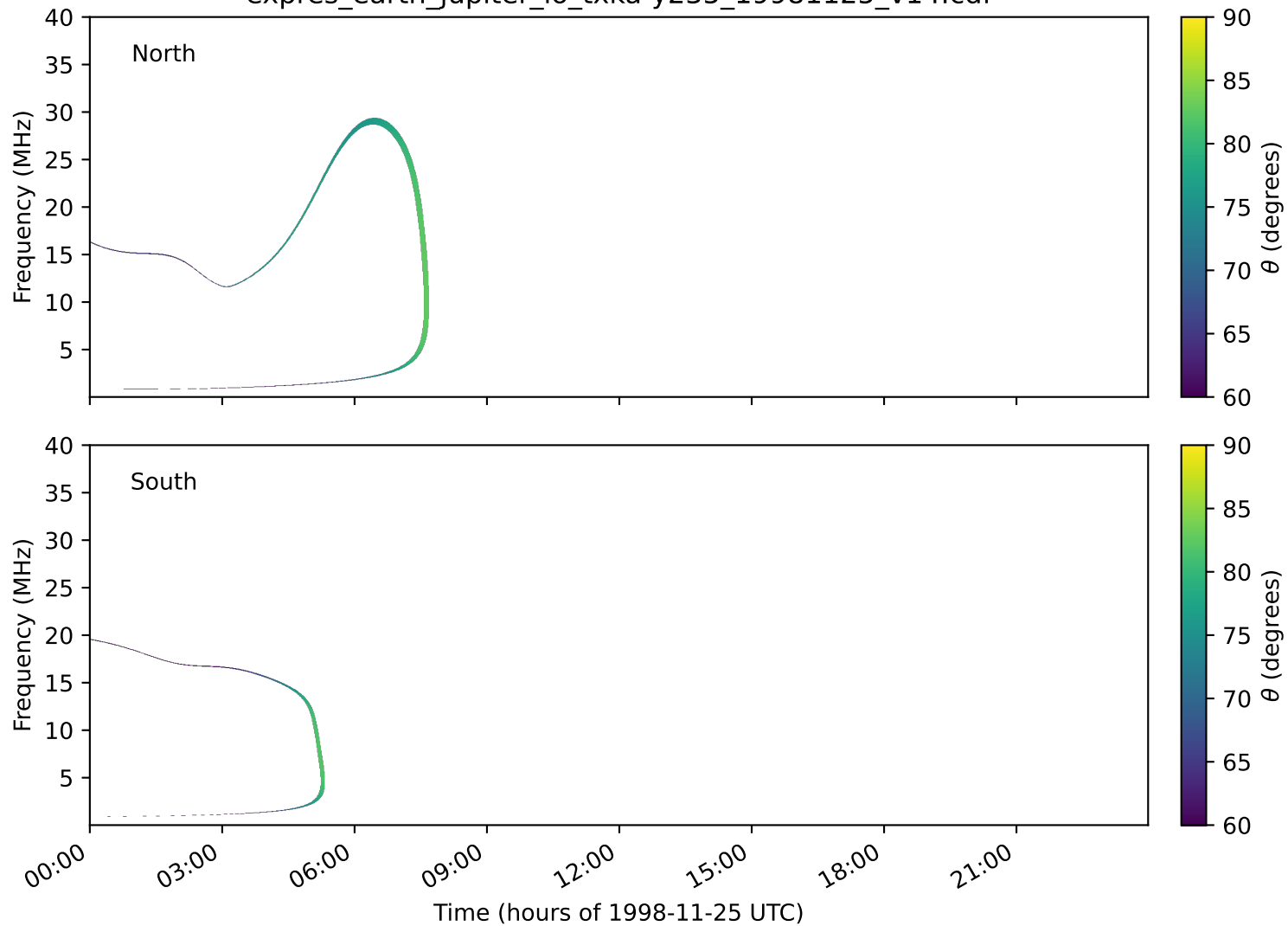
expres_earth_jupiter_io_txka-y235_19981125_v14.cdf
