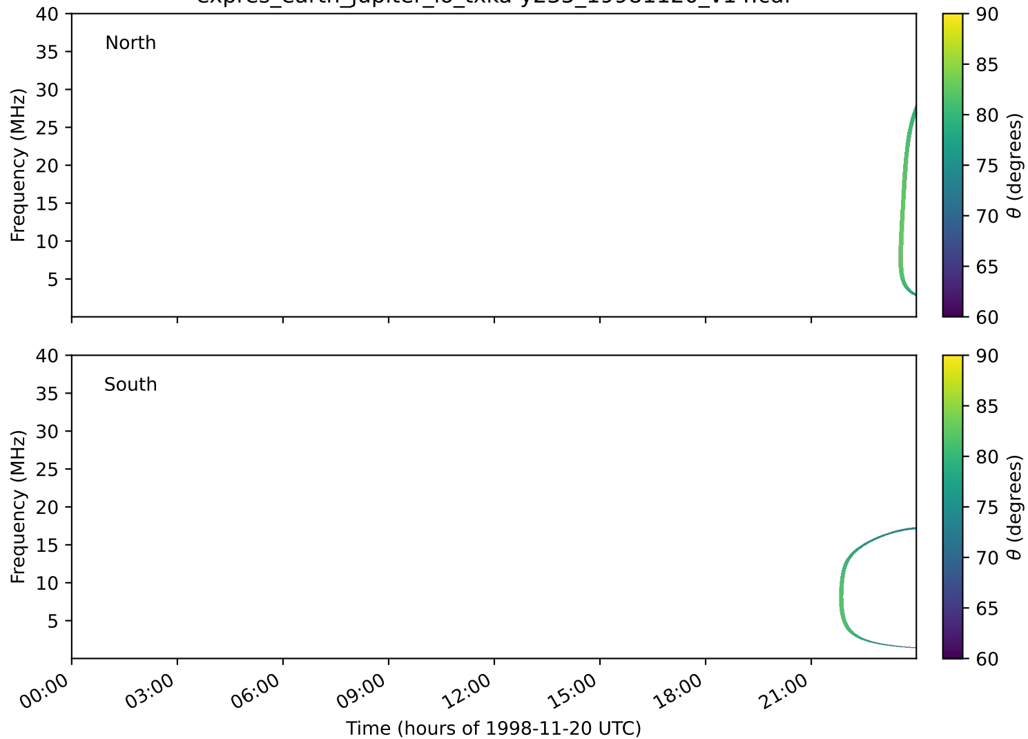
expres_earth_jupiter_io_txka-y235_19981120_v14.cdf
