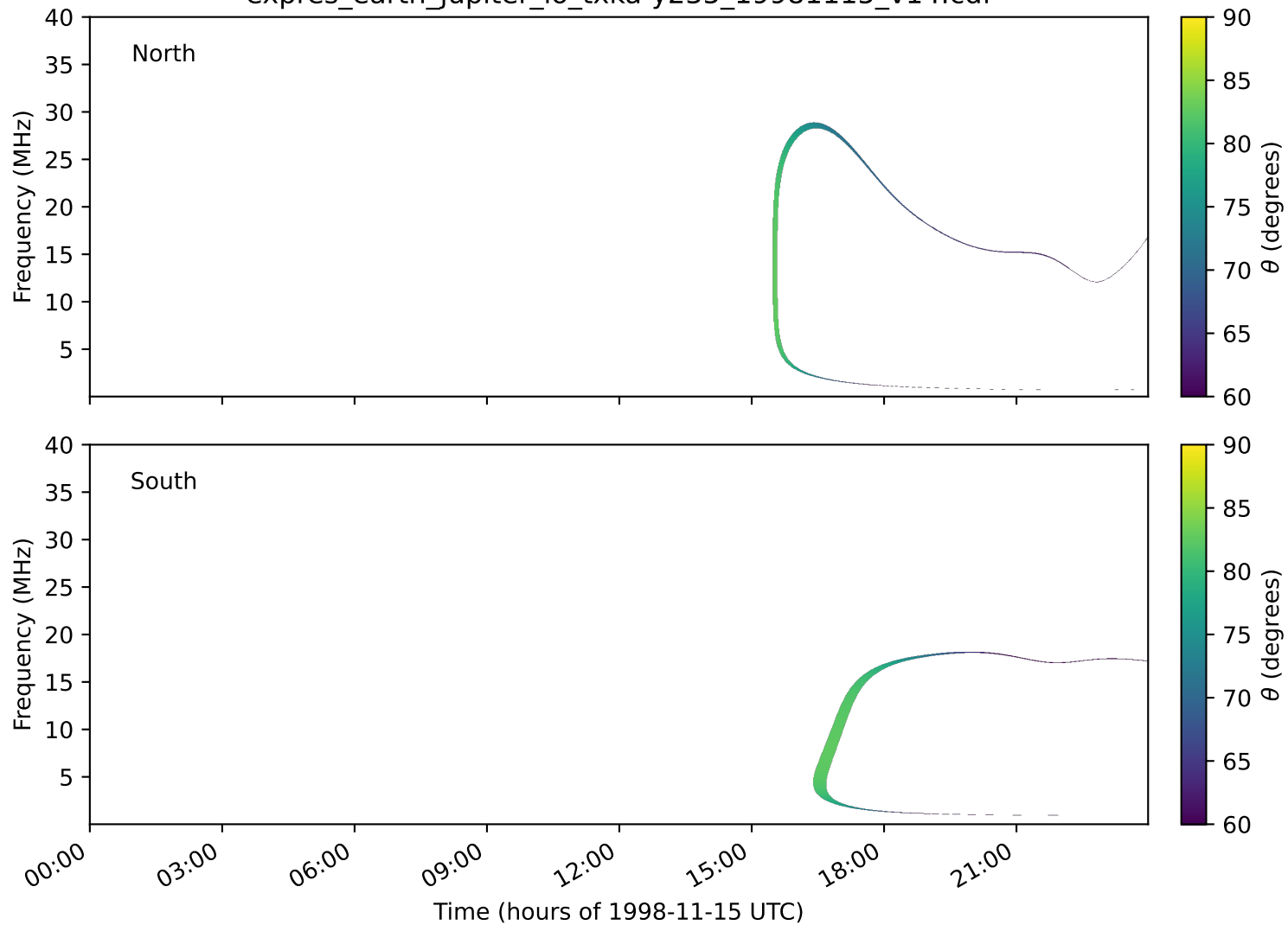
expres_earth_jupiter_io_txka-y235_19981115_v14.cdf
