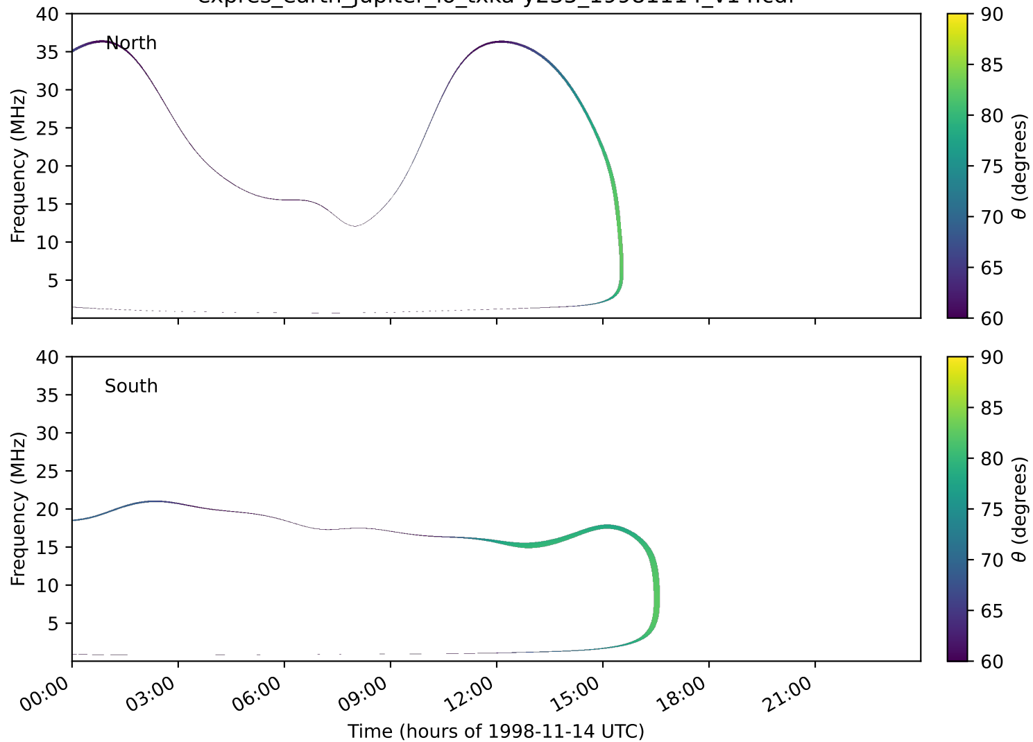
expres_earth_jupiter_io_txka-y235_19981114_v14.cdf
