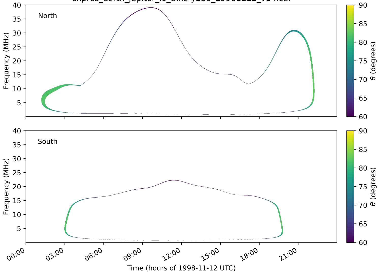
expres_earth_jupiter_io_txka-y235_19981112_v14.cdf
