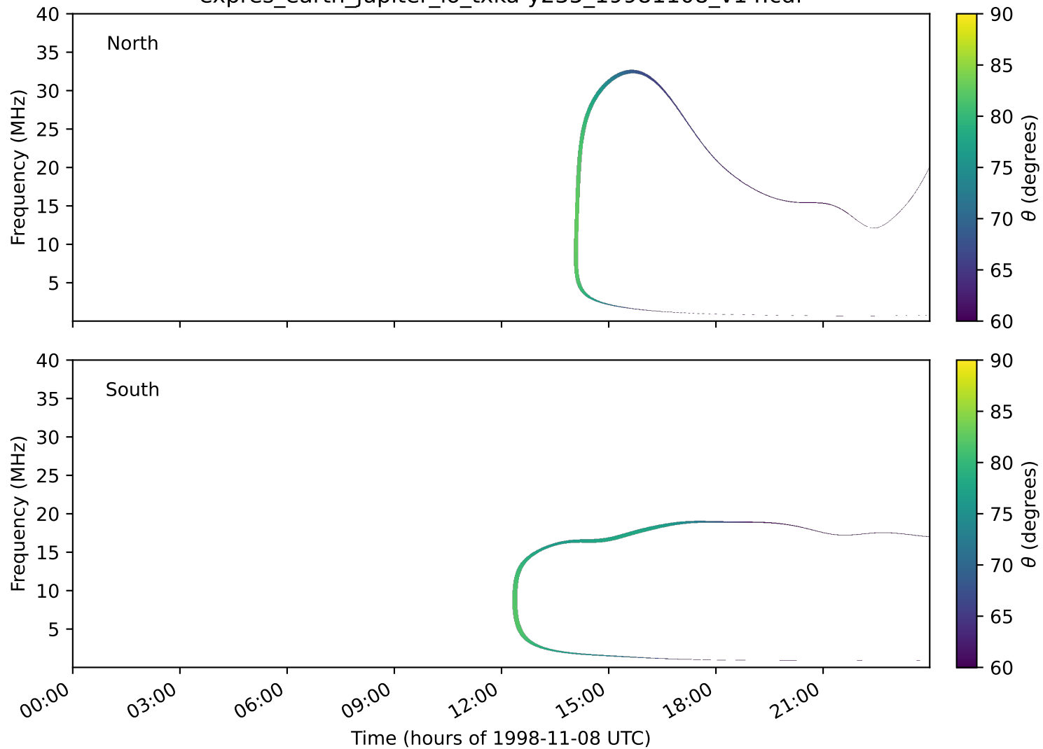
expres_earth_jupiter_io_txka-y235_19981108_v14.cdf
