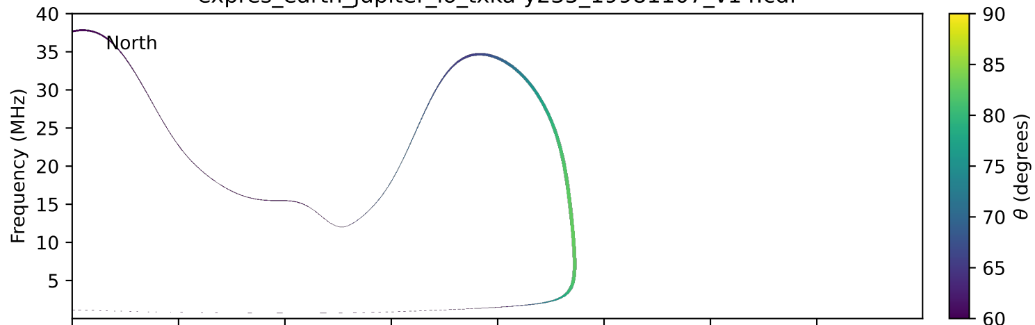
expres_earth_jupiter_io_txka-y235_19981107_v14.cdf
