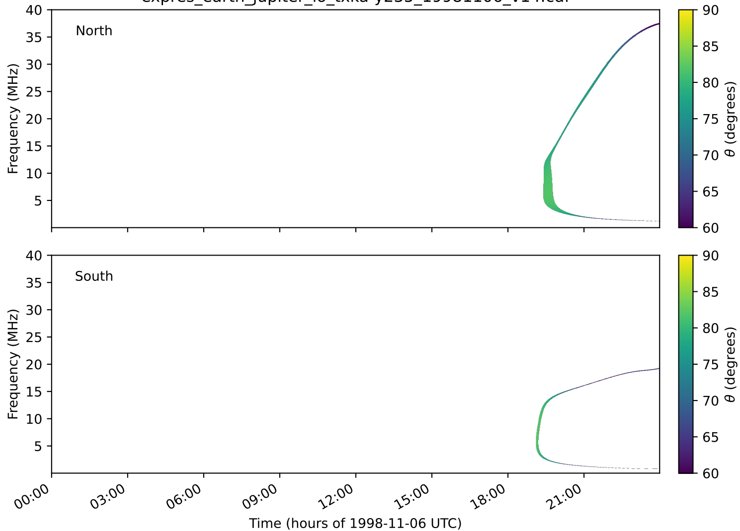
expres_earth_jupiter_io_txka-y235_19981106_v14.cdf
