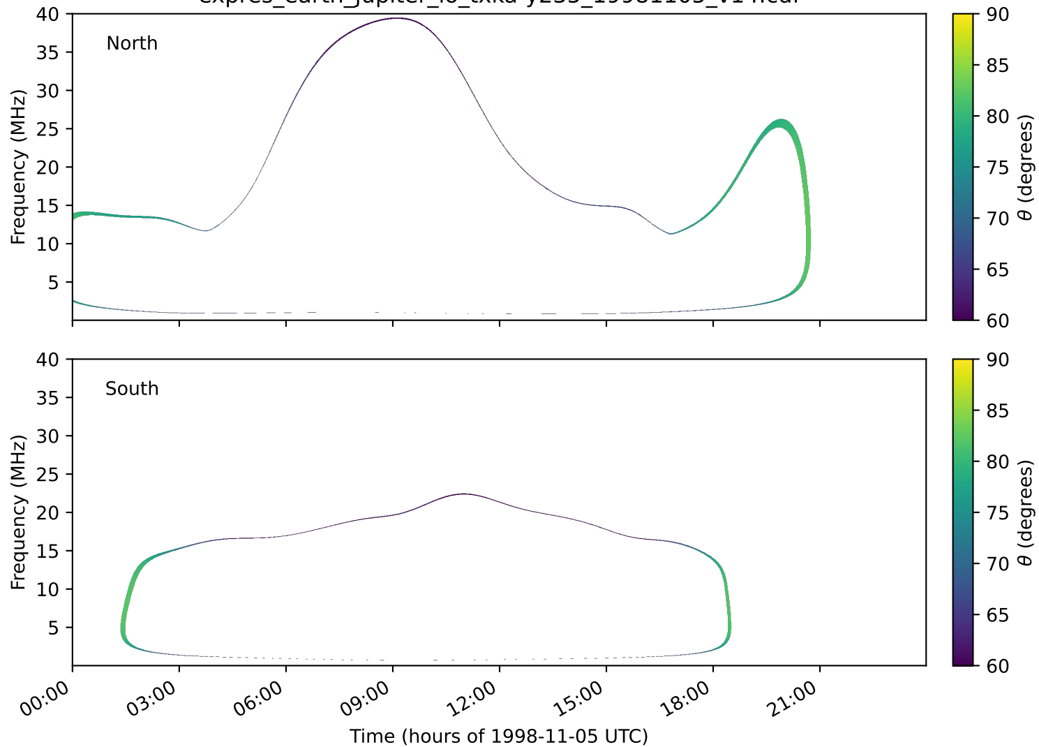
expres_earth_jupiter_io_txka-y235_19981105_v14.cdf
