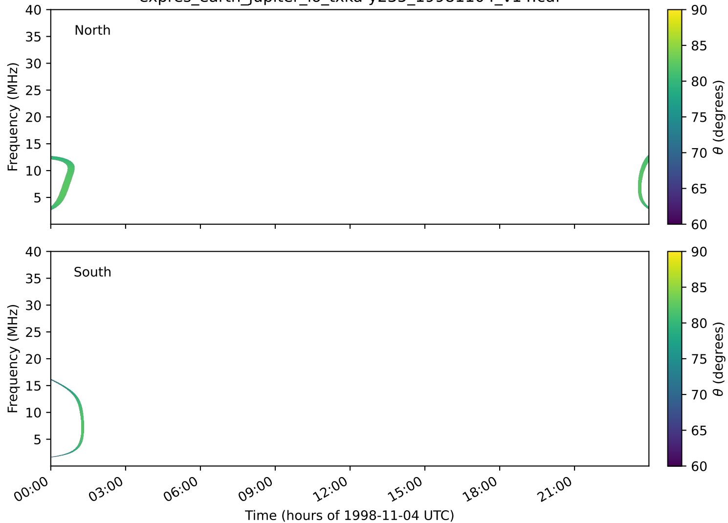
expres_earth_jupiter_io_txka-y235_19981104_v14.cdf
