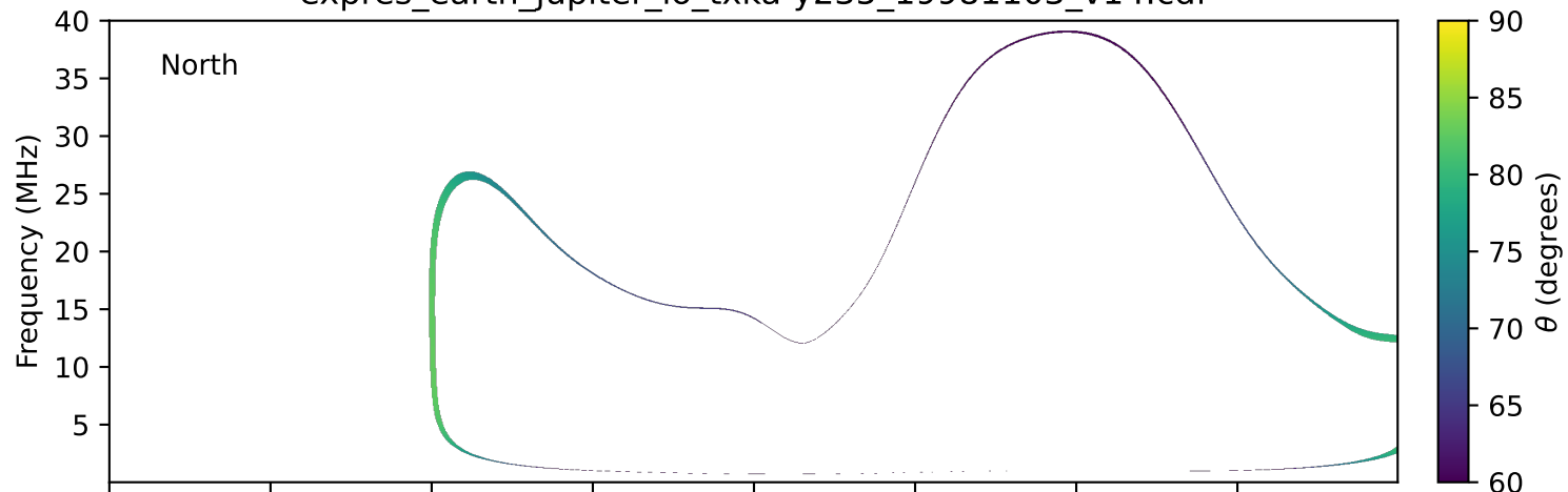
expres_earth_jupiter_io_txka-y235_19981103_v14.cdf
