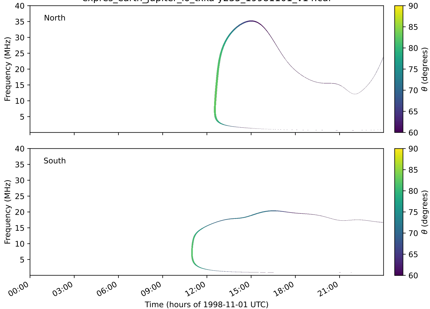
expres_earth_jupiter_io_txka-y235_19981101_v14.cdf
