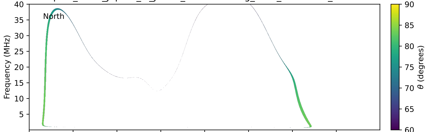
expres_earth_jupiter_io_jrm33_lossc-wid1deg_3kev_19981128_v11.cdf
