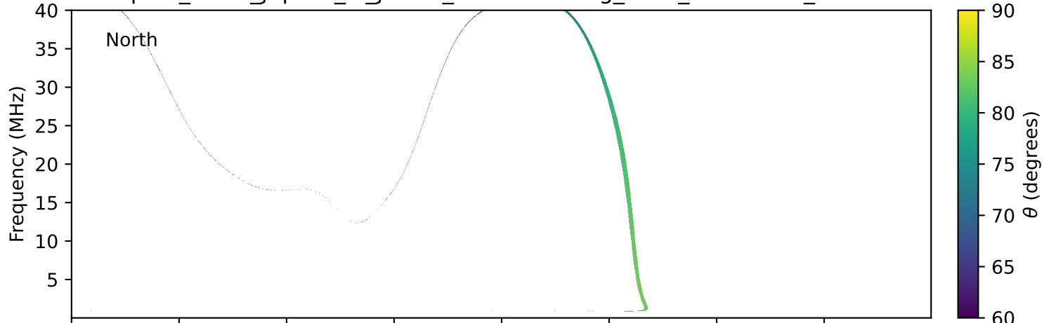
expres_earth_jupiter_io_jrm33_lossc-wid1deg_3kev_19981114_v11.cdf
