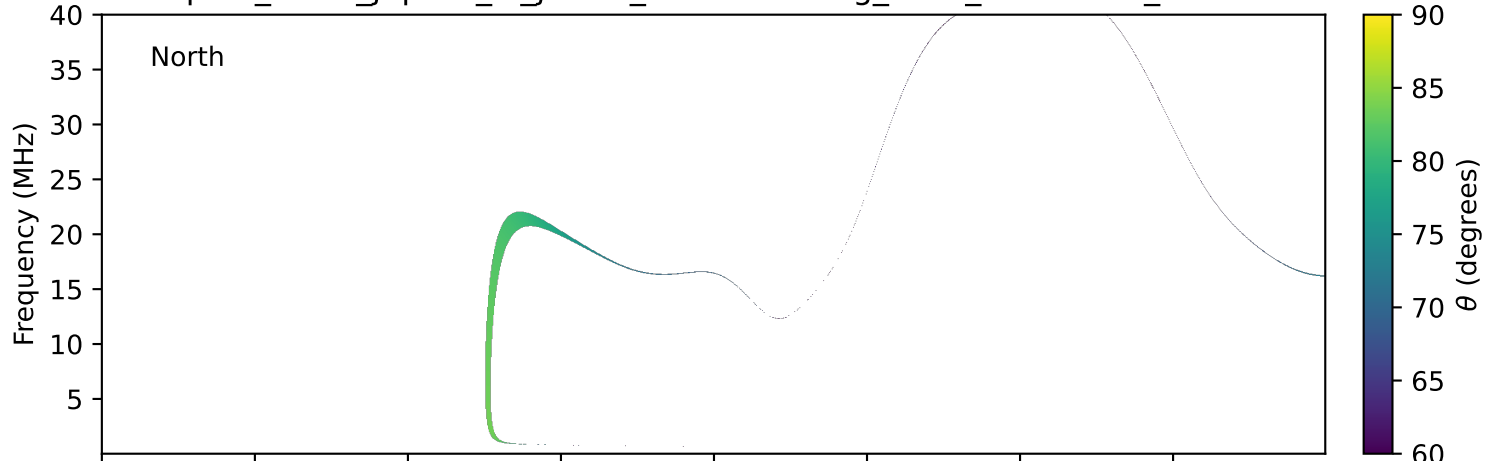
expres_earth_jupiter_io_jrm33_lossc-wid1deg_3kev_19981110_v11.cdf
