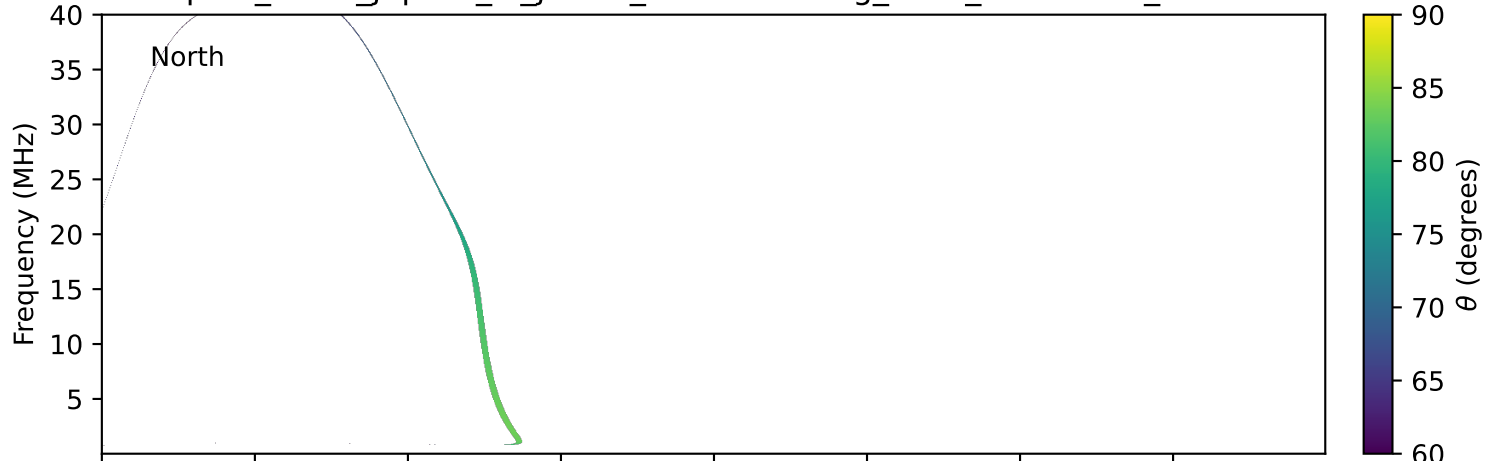
expres_earth_jupiter_io_jrm33_lossc-wid1deg_3kev_19981109_v11.cdf
