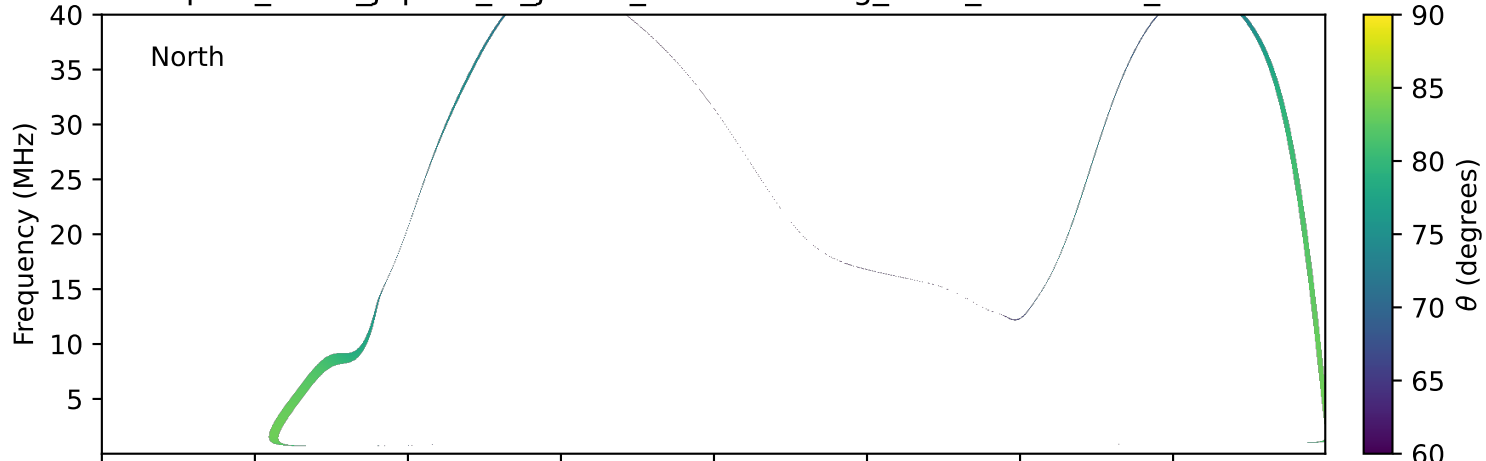
expres_earth_jupiter_io_jrm09_lossc-wid1deg_3kev_19981119_v11.cdf
