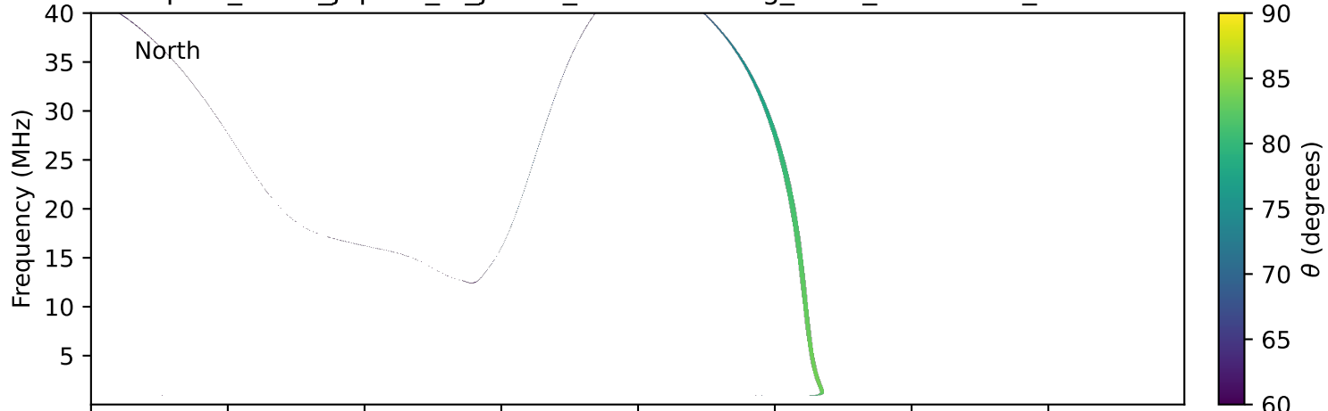
expres_earth_jupiter_io_jrm09_lossc-wid1deg_3kev_19981114_v11.cdf
