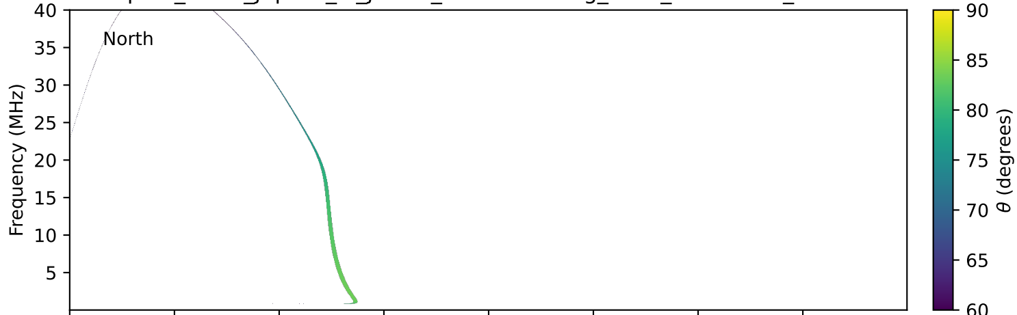
expres_earth_jupiter_io_jrm09_lossc-wid1deg_3kev_19981109_v11.cdf
