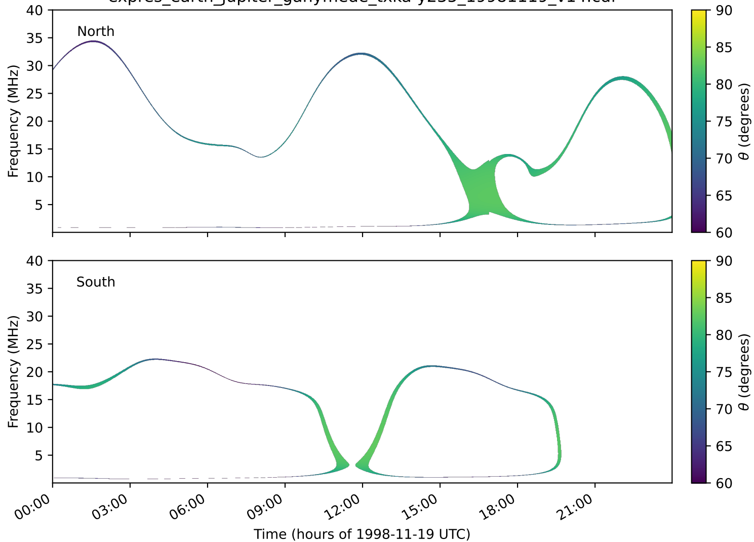
expres_earth_jupiter_ganymede_txka-y235_19981119_v14.cdf
