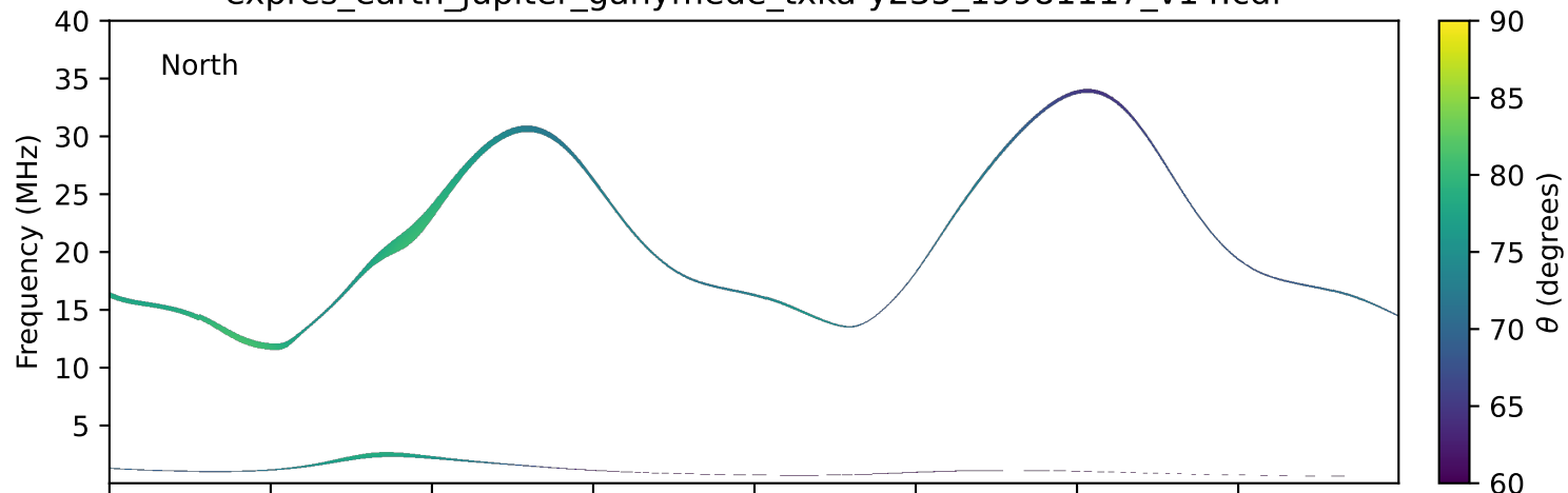
expres_earth_jupiter_ganymede_txka-y235_19981117_v14.cdf
