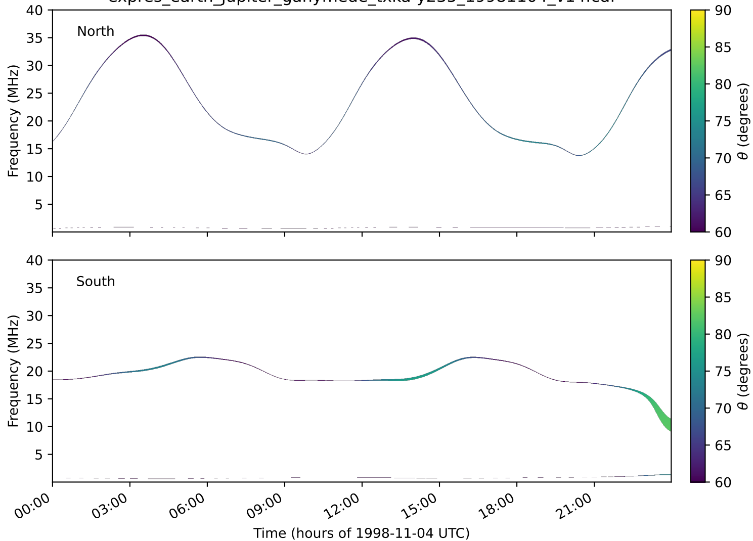
expres_earth_jupiter_ganymede_txka-y235_19981104_v14.cdf
