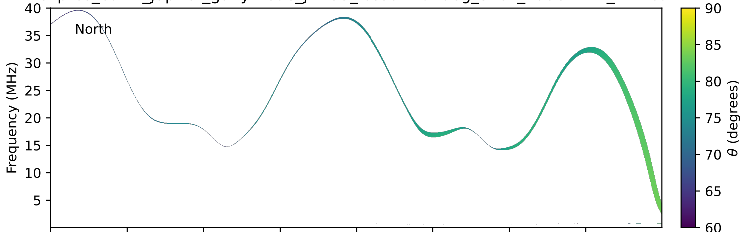
expres_earth_jupiter_ganymede_jrm33_lossc-wid1deg_3kev_19981112_v11.cdf
