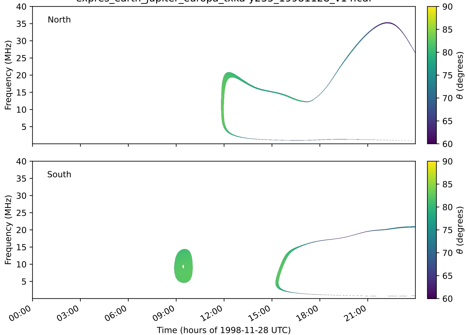
expres_earth_jupiter_europa_txka-y235_19981128_v14.cdf
