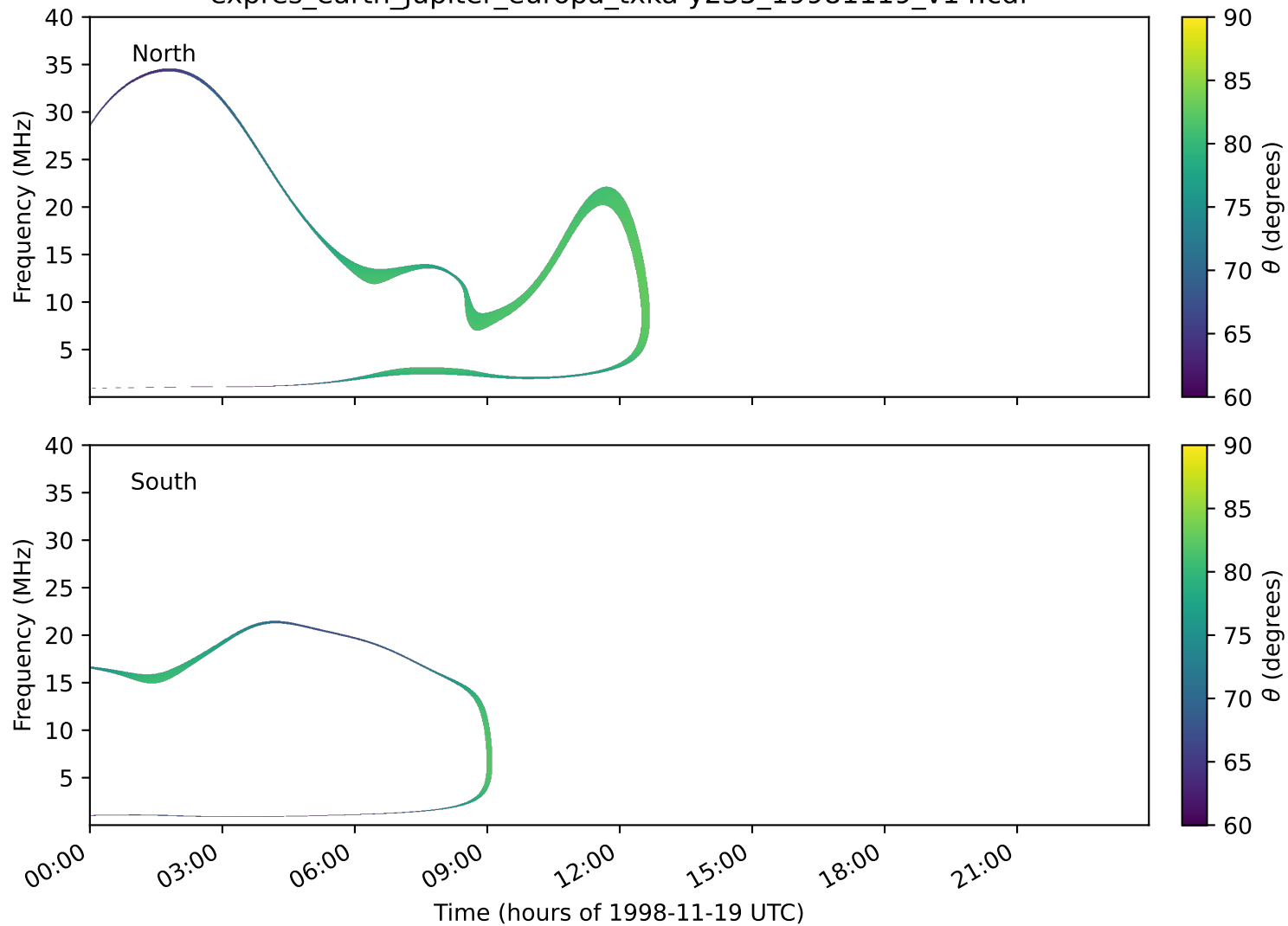
expres_earth_jupiter_europa_txka-y235_19981119_v14.cdf
