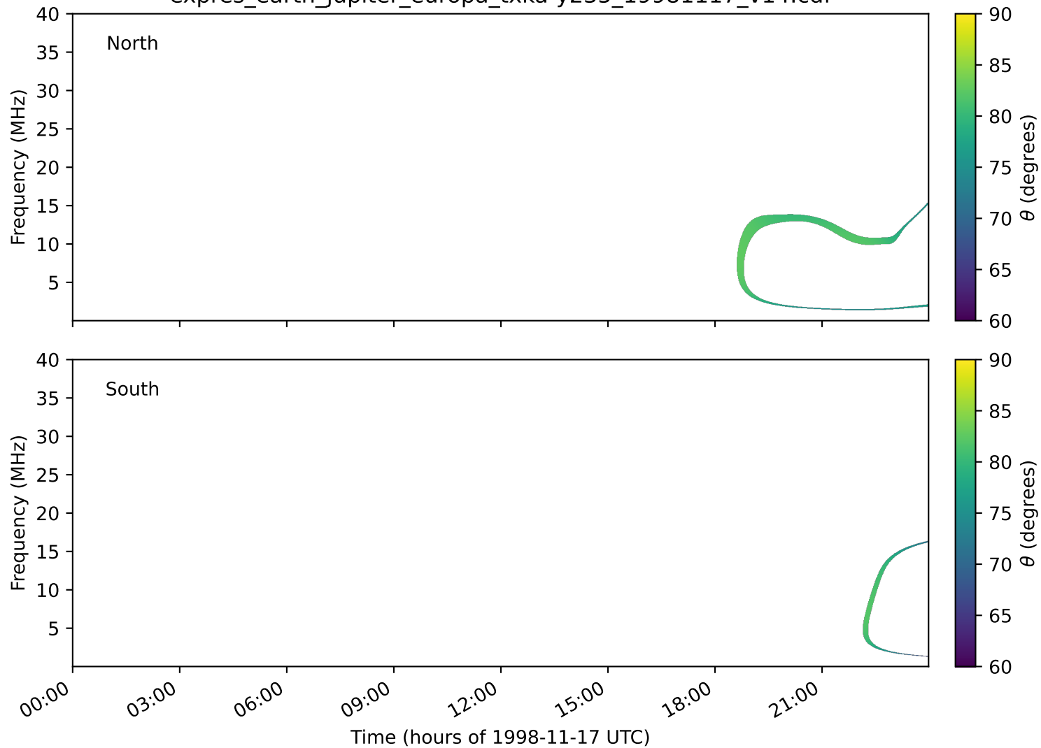
expres_earth_jupiter_europa_txka-y235_19981117_v14.cdf
