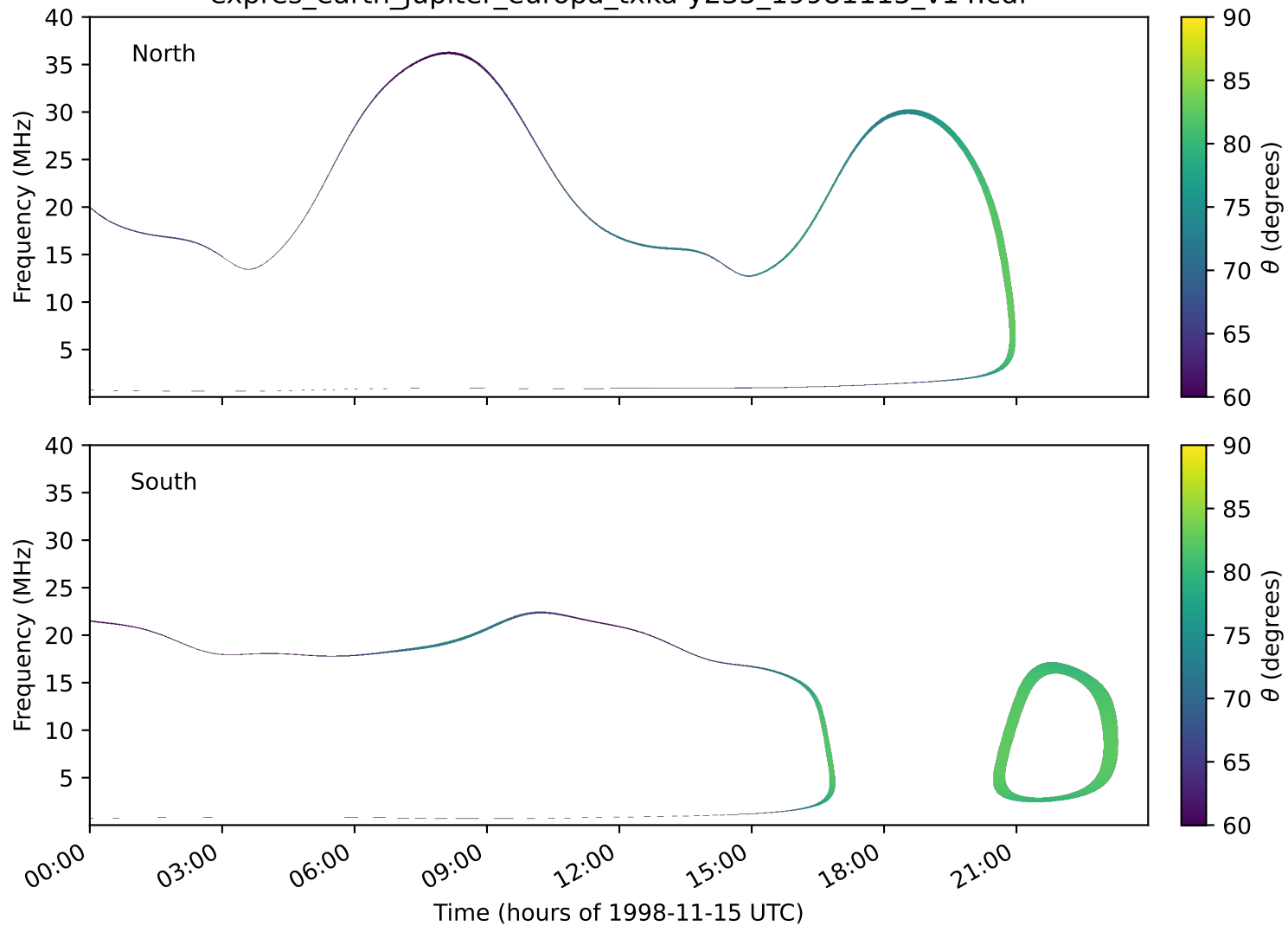
expres_earth_jupiter_europa_txka-y235_19981115_v14.cdf
