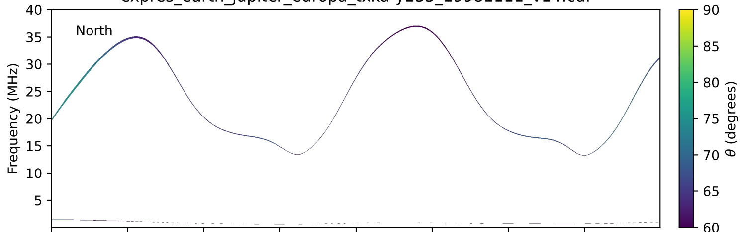
expres_earth_jupiter_europa_txka-y235_19981111_v14.cdf
