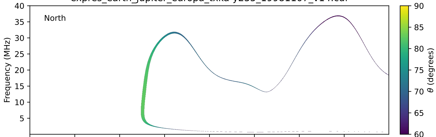
expres_earth_jupiter_europa_txka-y235_19981107_v14.cdf
