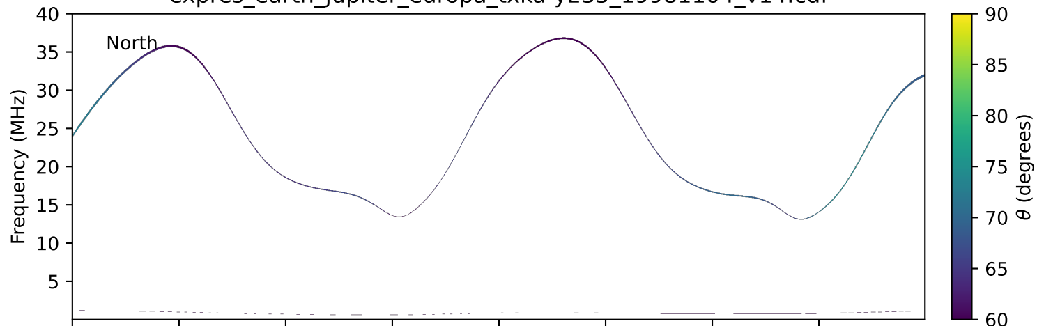
expres_earth_jupiter_europa_txka-y235_19981104_v14.cdf
