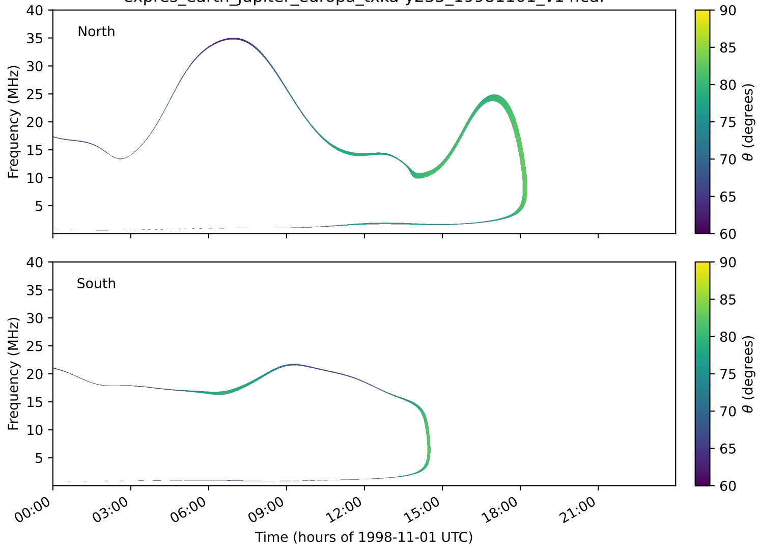
expres_earth_jupiter_europa_txka-y235_19981101_v14.cdf
