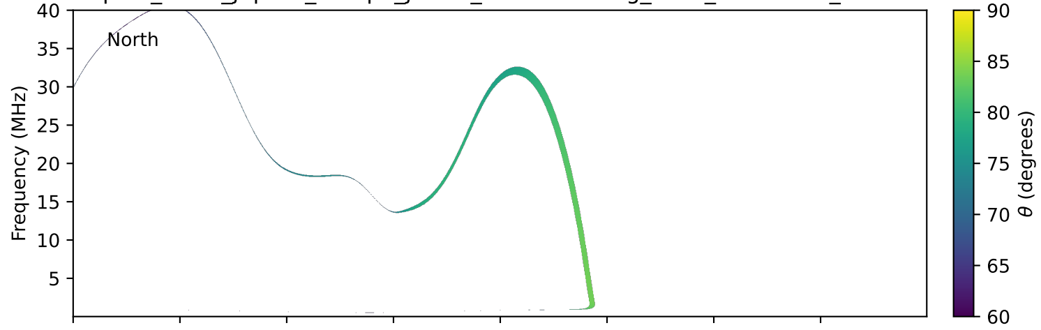
expres_earth_jupiter_europa_jrm33_lossc-wid1deg_3kev_19981126_v11.cdf
