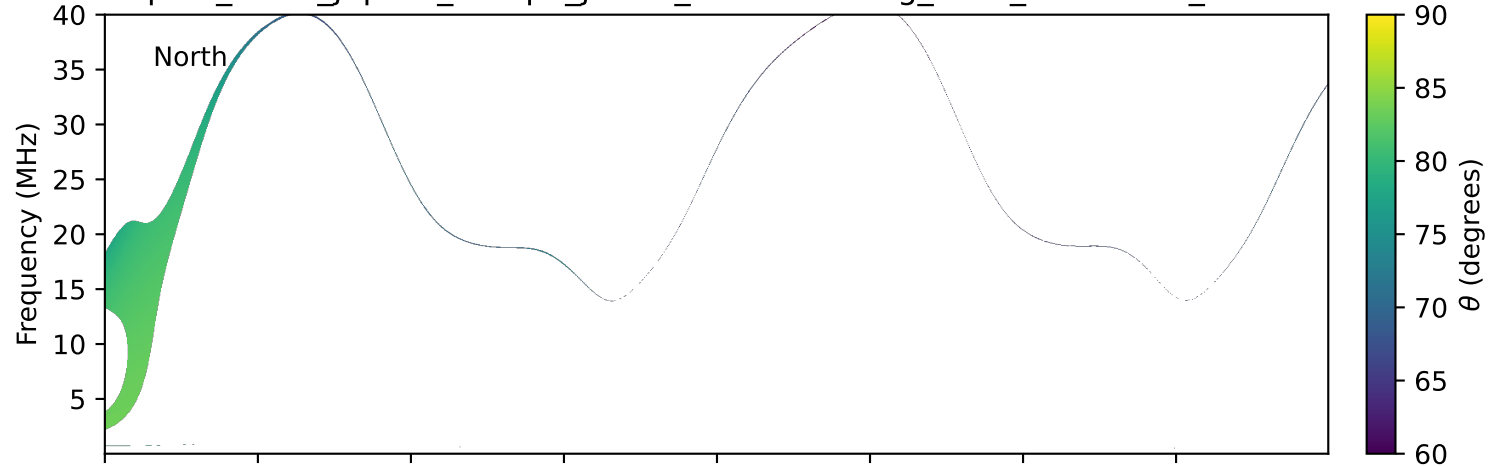
expres_earth_jupiter_europa_jrm33_lossc-wid1deg_3kev_19981118_v11.cdf
